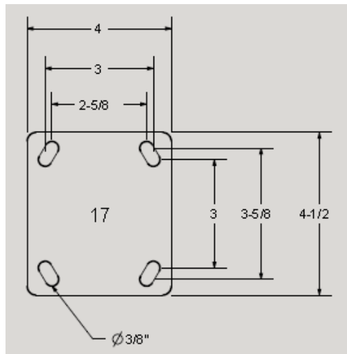
17 TOP PLATE
